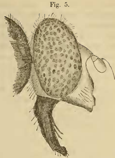
Helophilina taeniaticeps Beck.
