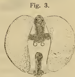
Paraphycus piceus Beck. 12:1
