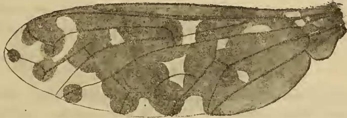
Argyromoeba perfecta Beck. Flügel 9:1.
