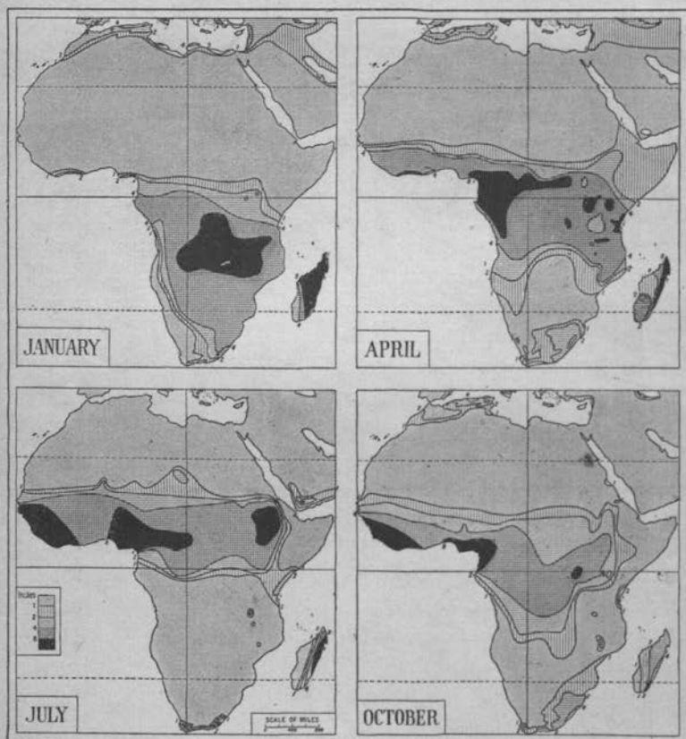
FIG. 3. Seasonal Rainfall.
