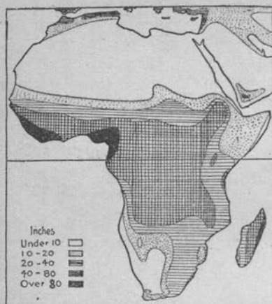
FIG. 1. Mean Annual Rainfall of Africa.
