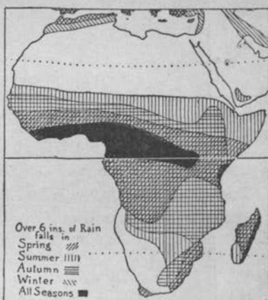
FIG. 2. Rainy Seasons in Africa.
