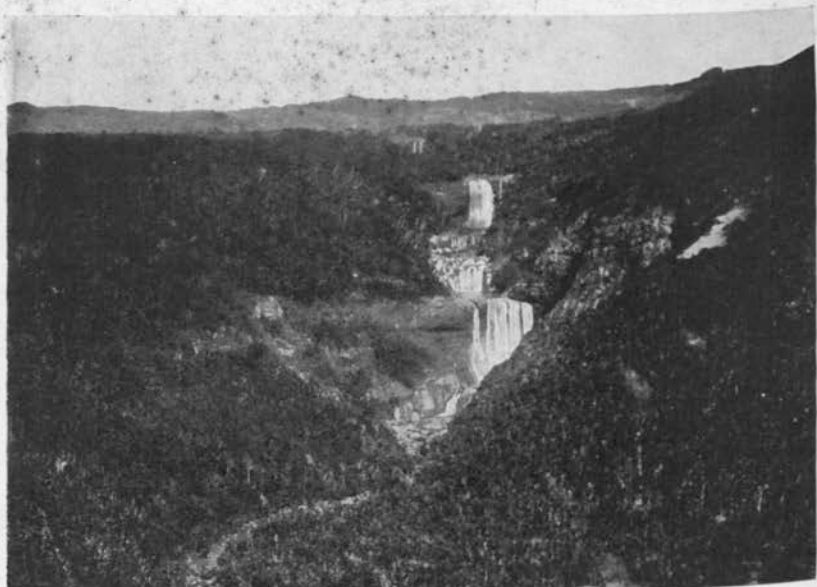
PLATE XXIX (a). CANYON AND FALLS NEAR VACOA, MAURITIUS
