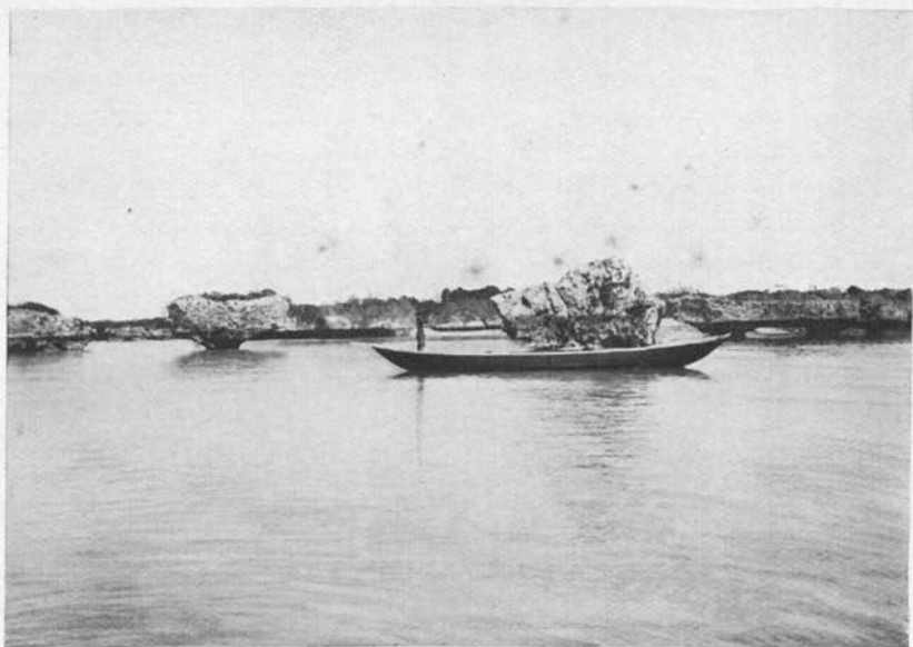
PLATE XXVIII (a). LAGOON OF ALDABRA, SHOWING EROSION OF ELEVATED CORAL ROCK
