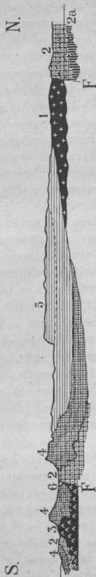
FIG. 10. Section from S. to N. approximately on 20° E. long.
