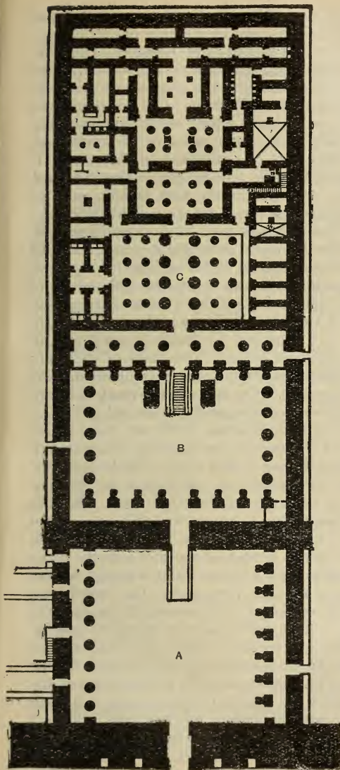
The Temple of Rameses III at Madînat Habû.
