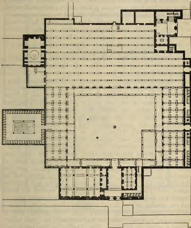
Plan of the Mosque Al-Azhar.
