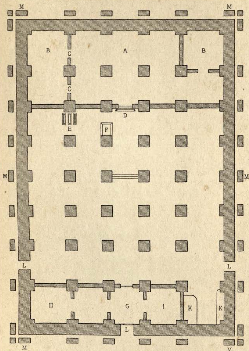
Plan of the Monolithic Church dedicated to the Saviour of the World (Madhanē 'Ālam) in the town of Lālibalā. From A. Raffray, Églises monolithes , Paris, 1882, Plate 3.
