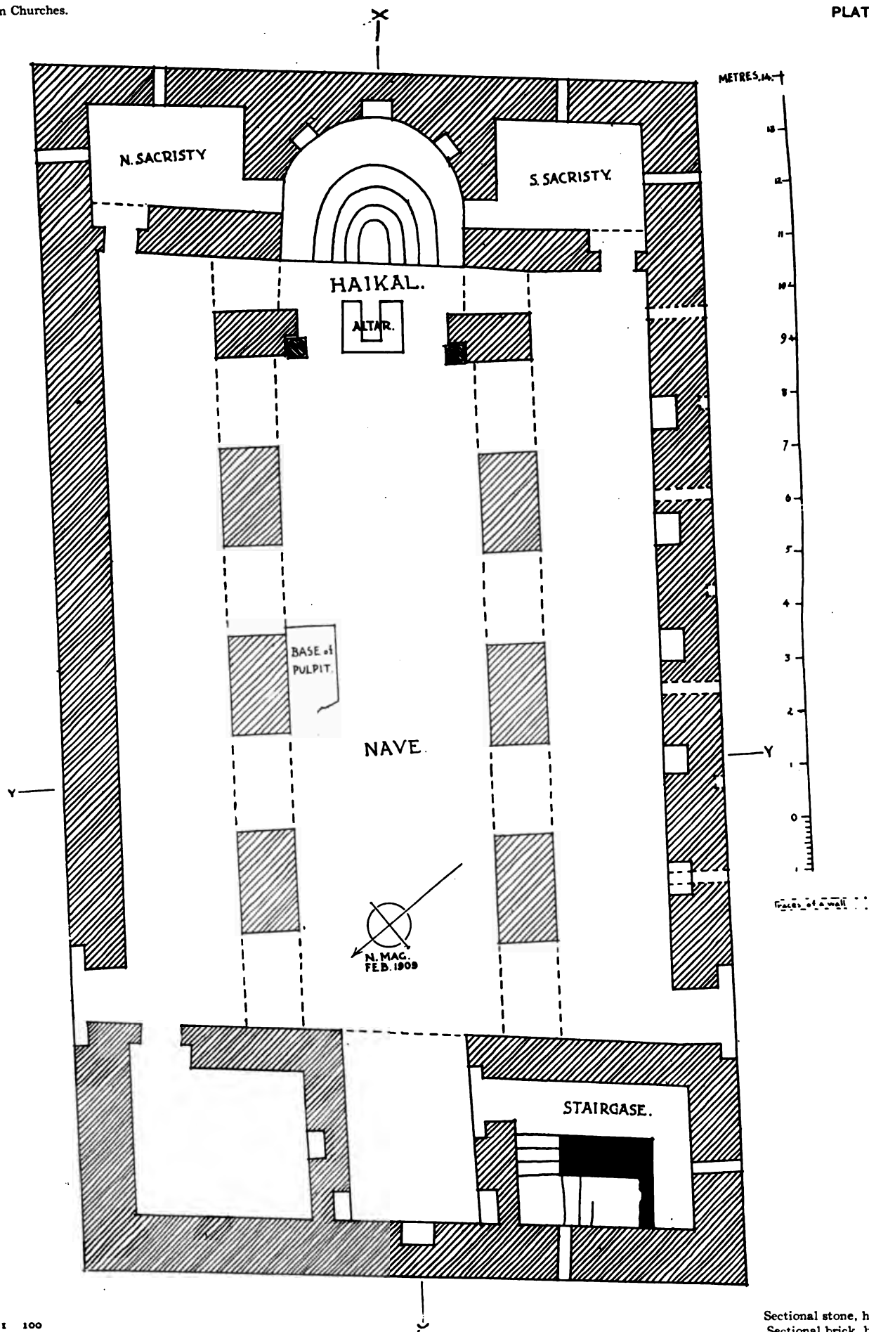
THE NORTHERN CHURCH NEAR ADDENDAN.
