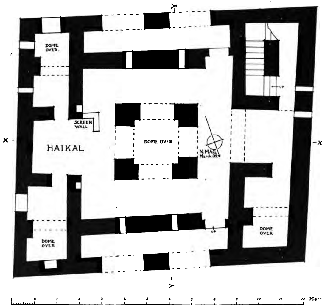
THE DOMED CHURCH NEAR ADDENDANA.
