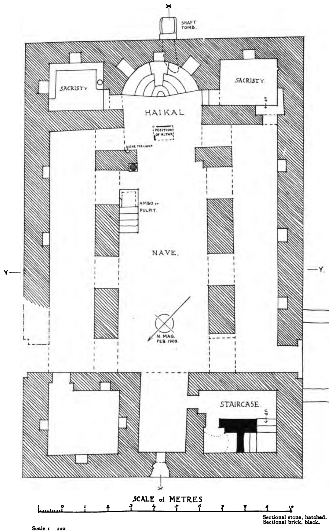
FARAS, THE NORTHERN CHURCH.
