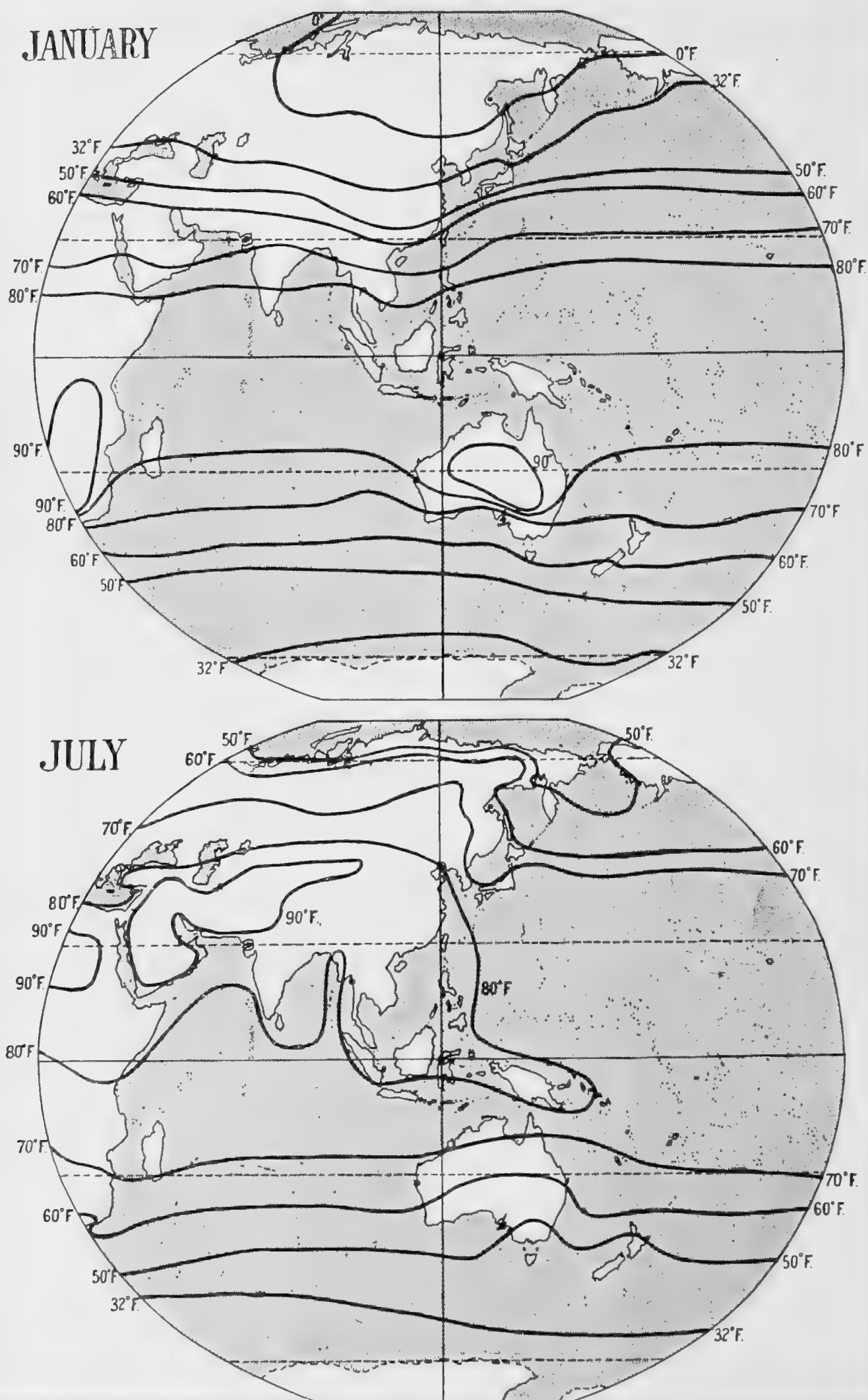
FIG. 16. Isotherms (mean temperature) over South-eastern Asia, &c., in January and July.
