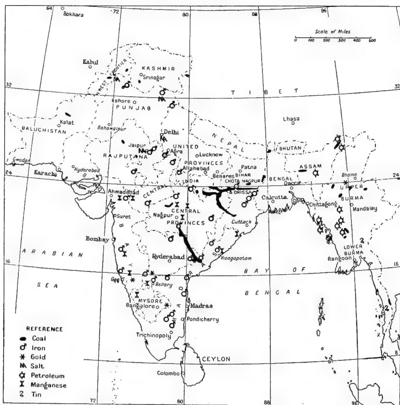
FIG. 8. Distribution of Economic Minerals in India.
