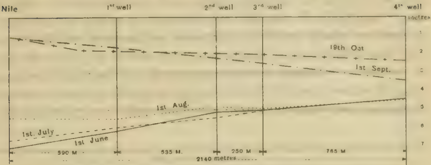
COMPARATIVE DIAGRAM OF WATER LEVEL OF THE NILE AND OF FOUR WELLS AT NAG HAMADI
