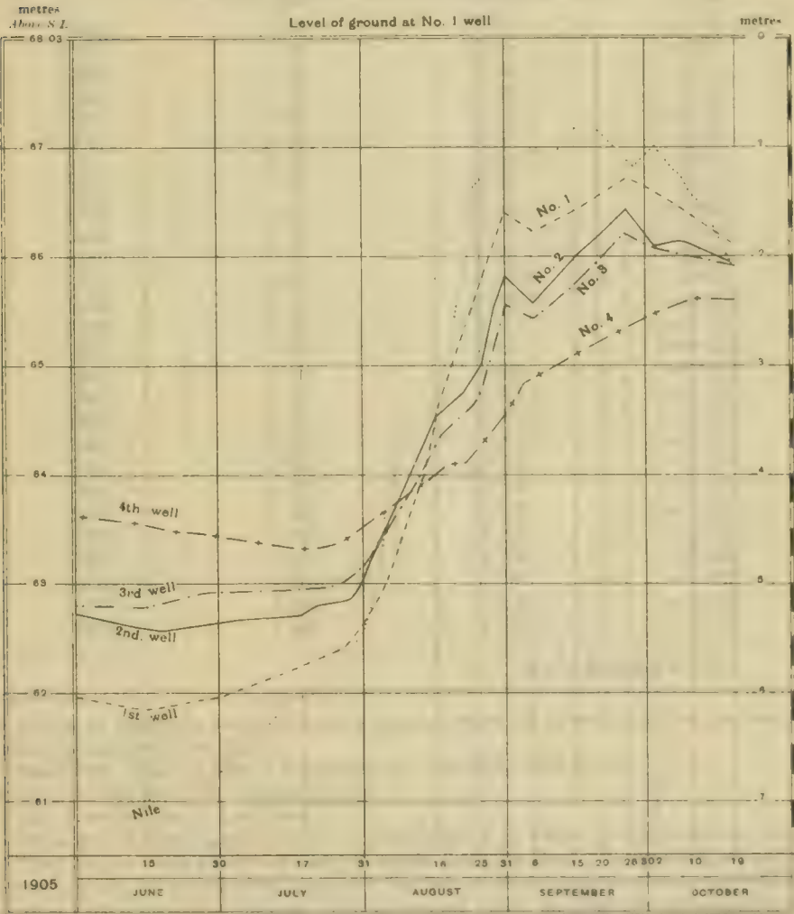
COMPARATIVE DIAGRAM OF WATER LEVEL OF THE NILE AND OF FOUR WELLS AT NAG HAMADI
