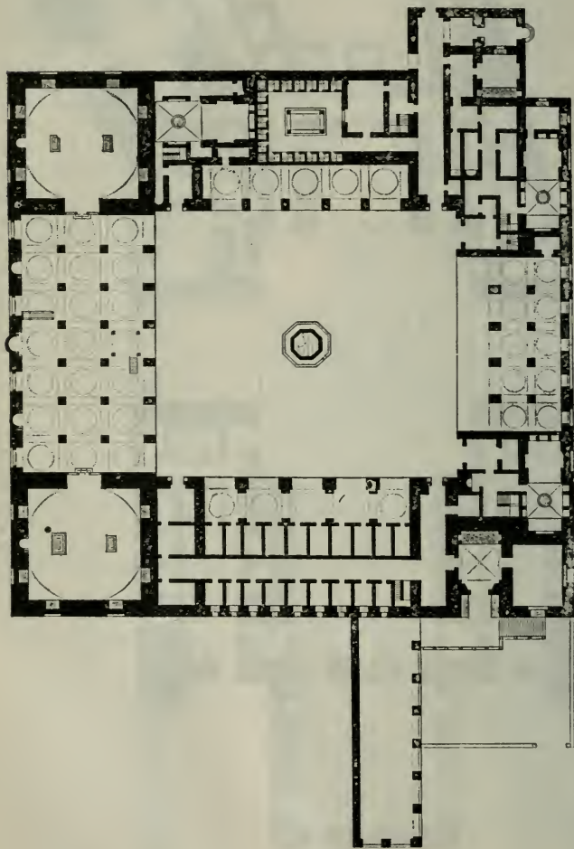
Plan of the Mosque of Barĳūk.
