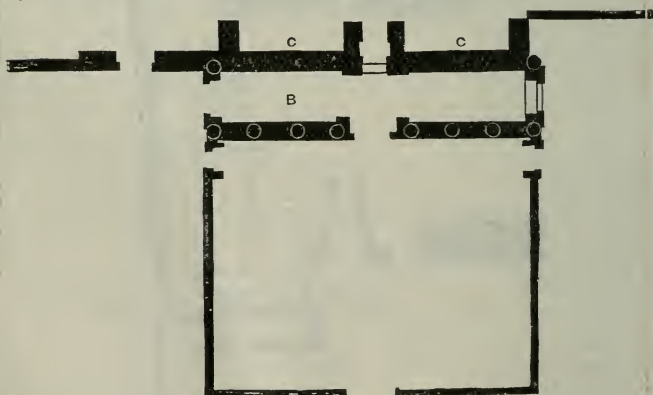
The Little Temple of Thothmes II at Madinat Habû.
